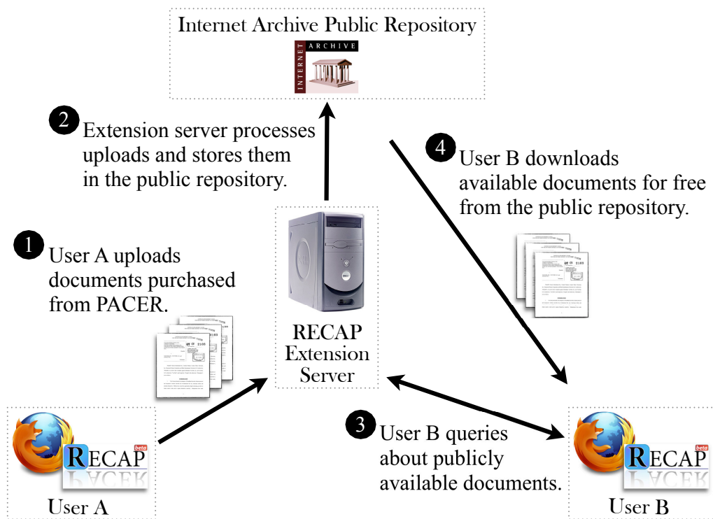
Figure 3.1: High-level architecture of the RECAP system.
